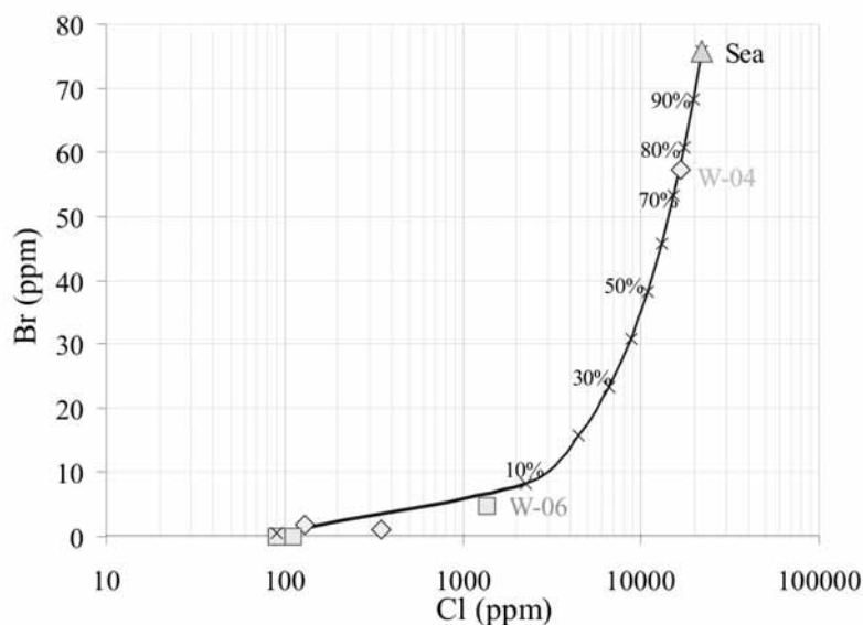
Figure 4.3: Tordera seawater-freshwater \text{Cl}^-/\text{Br}^- mixing model. Diamonds and squares shows three hydrochemical lectures on depth of W-04 and W-06 where percentage of seawater could be derived. For specific location of W-04 and W06 see Figure 4.5. or Figure 4.10. (Modified form Soler et al. , 2006).
