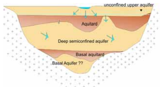
Figure 4.2: Tordera hydrogeologic conceptual model composed by: an upper free aquifer, a deep semiconfined aquifer, and a basal aquifer. Arrows show an ideal water flux, river is mainly influent where vertical recharge flows from the upper aquifer to the deep aquifer and from the upper basin aquifer zones.
