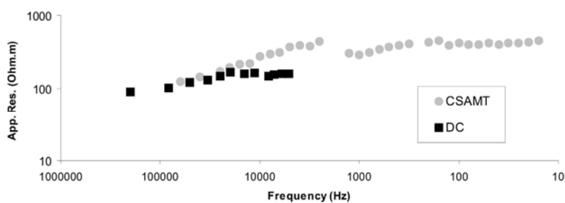
Figure 5.11: F4 DC resistivity data (black) in the frequency domain and AMT data (grey).
