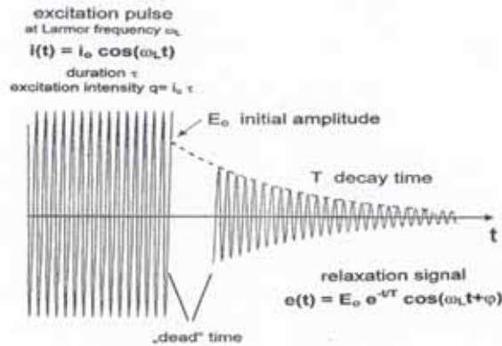
Figure 2.11: Input and output signals of NMR (from Yaramanci et al. , 2005).
