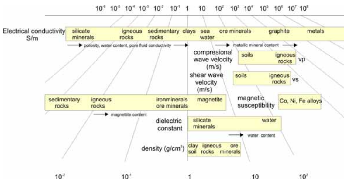
Figure 2.3: Scale ranges of rock properties, electrical conductivity, s and p-wave velocity, magnetic susceptibility, dielectric constant and density. (Modified from The Berkeley course on applied geophysics).
