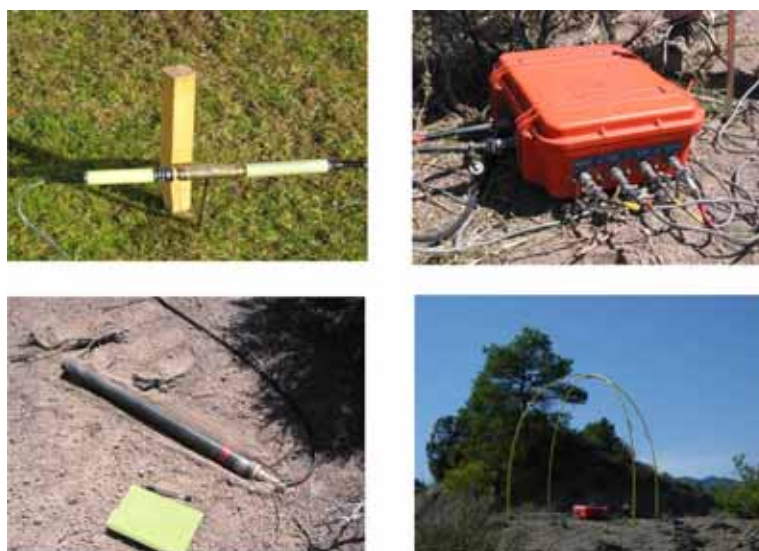
Figure 3.6: Pictures illustrating the different components of the StrataGem system. From left to right and top to bottom is shown an electrode, the AEF receiver box, an induction coil, and the controlled source.
