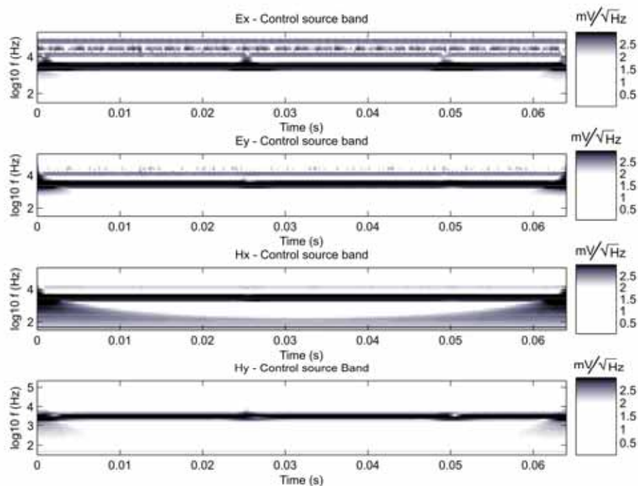
Figure 3.7: Frequency domain spectral analysis based on the Morlet wavelet transform showing the 4 AMT data components (courtesy of C. Arango.). The dominant frequency appear as a high amplitude band at one specific frequency (black line), that corresponds to one of the fourteen frequencies transmitted by the controlled source.
