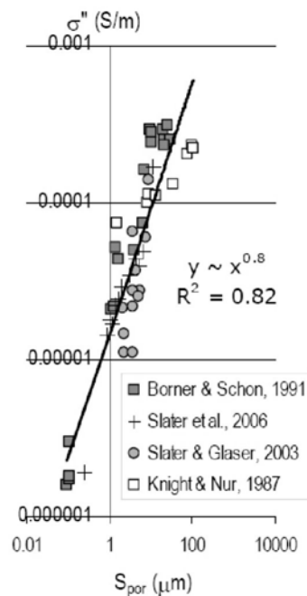
Figure 2.17: Compilation of measurements of specific porous surface area S_{por} and imaginary electric component \sigma'' from different materials and studies, showing a consistent relationship (from Slater, 2006).
