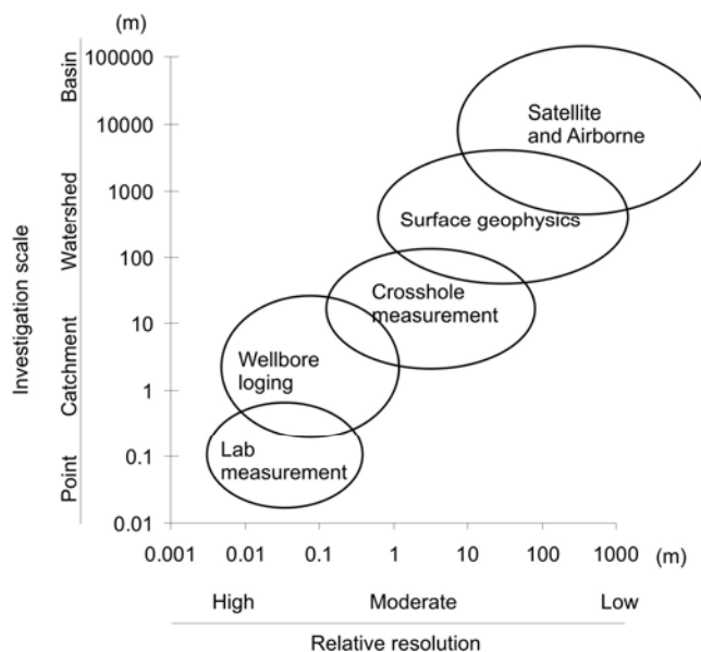
Figure 2.1: Schematic diagram of field geophysical length scale resolution and study objective scale (Modified from Rubin and Hubbard, 2005).
