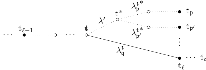
Figure 6.3: Non-optimised tree with potentially unbounded prime ideals, \phi_{\ell, \mathfrak{q}} \neq \phi(\mathfrak{p}, \mathfrak{p}') .
