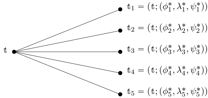
Figure 2.10: Segment of an optimised tree starting from \mathfrak{t} .
