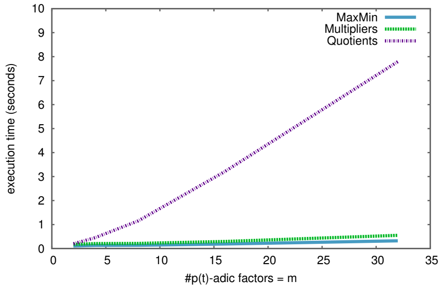
Figure 7.14: Running time for maximal order p(t) -basis computation defined by polynomials A_{t^2+4,n,28}^m(x) with n \cdot m = 64 , m \in \{2, 4, 8, 32\} .
