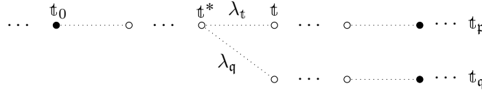
Figure 6.4: S_{\mathfrak{t}} is precomputable for \mathfrak{t} in the non-optimised tree.
