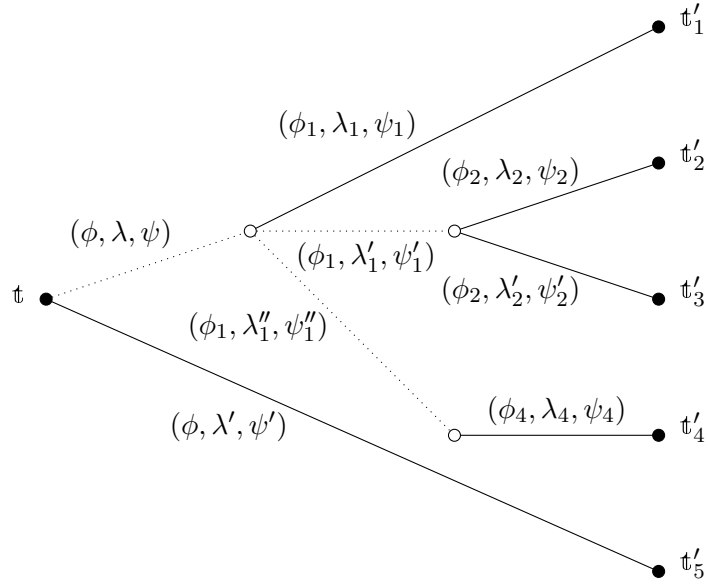
Figure 2.9: Segment of a non-optimised tree starting from \mathfrak{t} .
