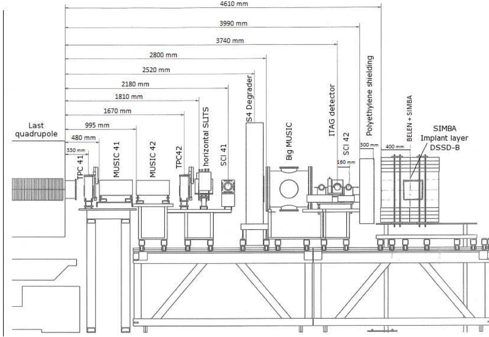
Figure 2.6: Schematic figure of the experimental setup at the S4-hall. (Adapted figure from S410 experiment team)
