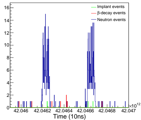
Figure 3.21: Implant, \beta -decays and neutron events in a random interval of time where it can be appreciated the bunch of mostly background neutrons correlated with the beam spill.
