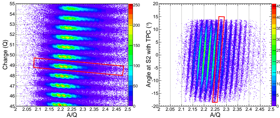
Figure 2.8: Left: PID before the correction where an element, in the fission fragments region is selected. Right: Measured angle along the A/Q of isotopes of the selected element. The selection corresponds to the isotope chosen for the angle correction calculation.
