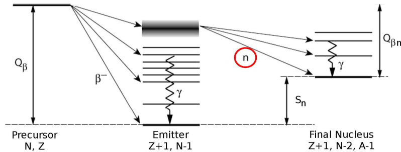
Figure 1.1: \beta -delayed neutron emission scheme.
