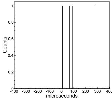
Figure 4.7: \beta -neutron correlation events during the 213 Tl implant- \beta correlation time within an area of 9 mm 2 .
