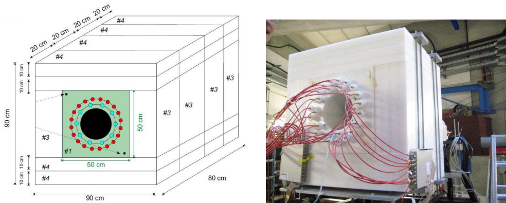
Figure 3.16: Left: Scheme of the 30 3 He counters distributed in the polyethylene matrix. Right: Image of BELEN detector during the experiment. Red cables connect the counters and the preamplifiers.
