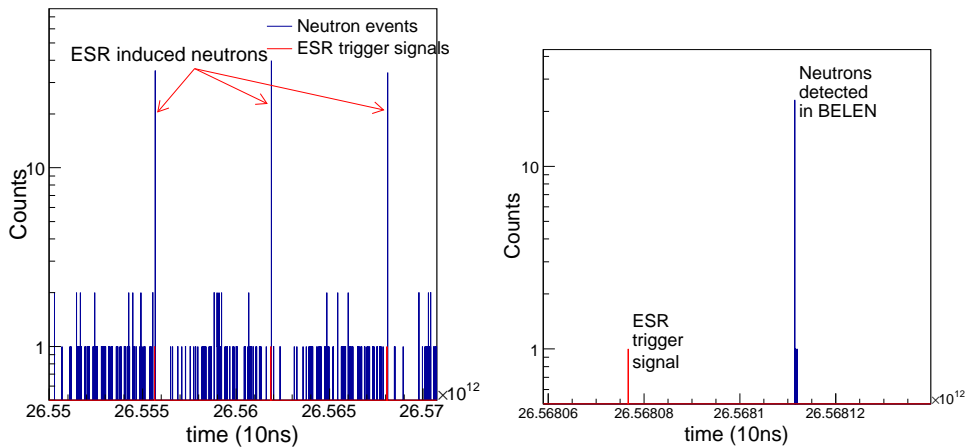
Figure 3.20: Left: Example of several ESR trigger signals (red) and neutrons (blue) for a random interval of time. It can be observed the correlated neutrons appeared just 347.2 ms after the ESR trigger. The right figure shows a zoom where the ESR trigger signal (in red) can be observed together with its correlated bunch of neutrons.
