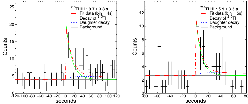
Figure 4.11: Implant- \beta correlation diagrams of 215 Tl (left) and 216 Tl (right), using a correlation area of 25 mm 2 .
