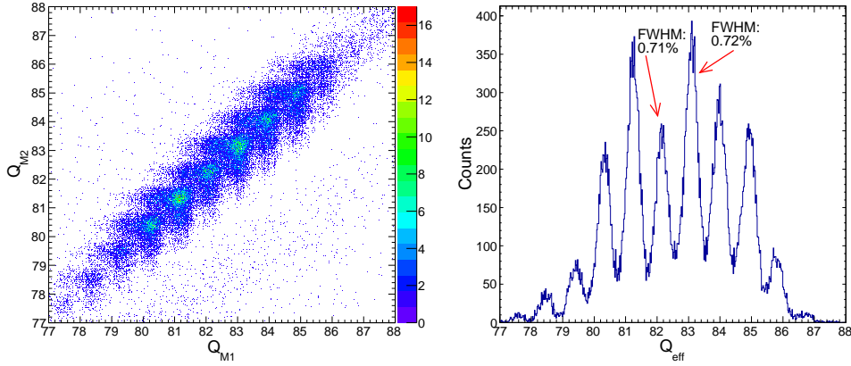
Figure 2.17: Left: Correlation of the charge calculated from the information of both MUSIC ( Q_{M1} and Q_{M2} ). Right: Determined Q_{eff} statistics for the amount of events tracked by the FRS in the ^{211}\text{Hg} setting.
