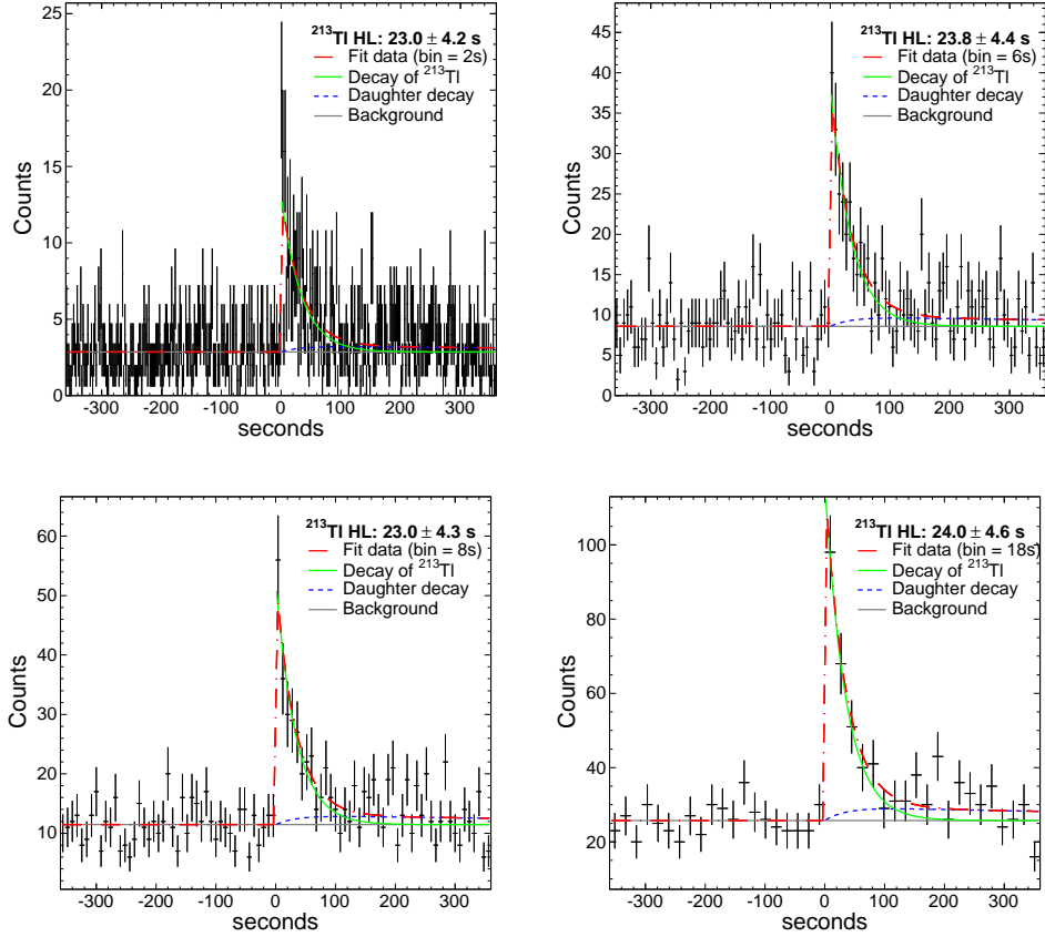
Figure 4.5: ^{213}\text{Tl} half-life fits of implant- \beta events off-spill with a 9 \text{ mm}^2 correlation area around the implant. Top-left with a binning time width of 2 s, top-right 6 s, bottom-left 8 s and bottom-right 18 s.
