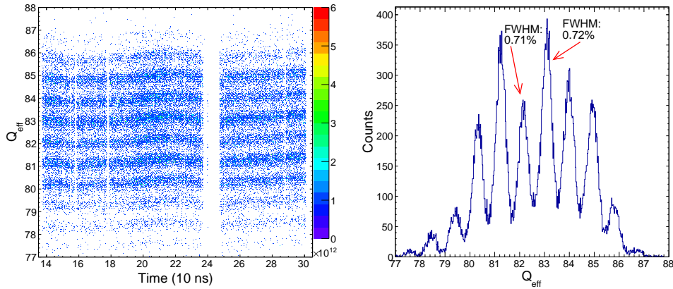
Figure 2.18: Left: Correlation of Q_{eff} along the time (before the drift correction). Right: Projection of the vertical axis, corresponding to the Q_{eff} accumulated during the ^{211}\text{Hg} setting.
