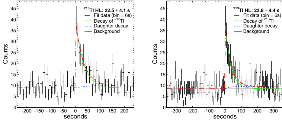
Figure 4.6: ^{213}\text{Tl} half-life fits varying the correlation time-range.
