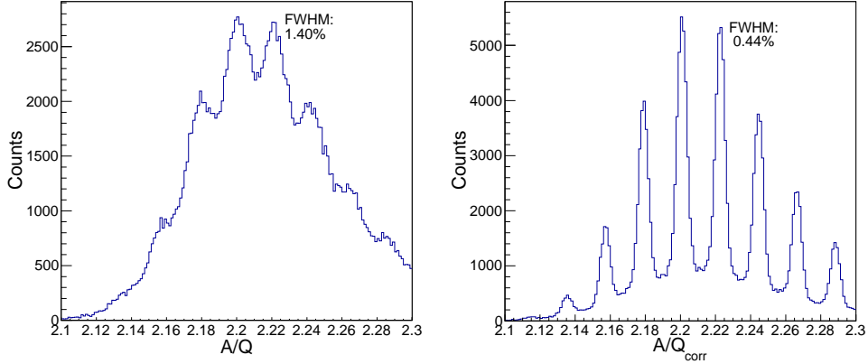
Figure 2.10: Projection of isotopes of a particular element in the region of the fission fragments from figures 2.8-left and 2.9-right. The indicated FWHM values show the resolution improvement for a selected isotope, with a determined raw charge of Q = 49 and a raw A/Q centered between A/Q = 2.22 and A/Q = 2.23 . Left: Before the angle correction. Right: After the correction.
