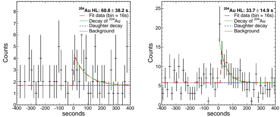
Figure 4.17: ^{204}\text{Au} implant- \beta diagrams. Left: correlation area of 9 mm 2 . Right: correlation area of 25 mm 2 and extended with all \beta -particles including those inside the spill. See text for details.
