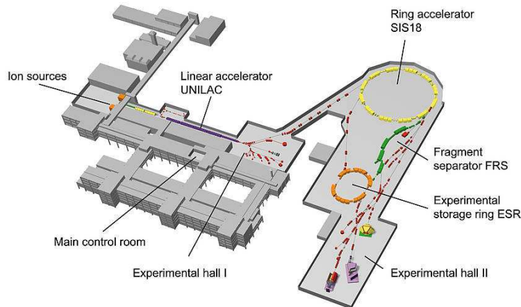
Figure 2.1: GSI facility scheme, which comprises the linear accelerator UNILAC, the SIS-18 synchrotron, the Fragment Separator (FRS), the Experimental Storage Ring (ESR) and a number of experimental halls to host the detection systems for each experiment.
