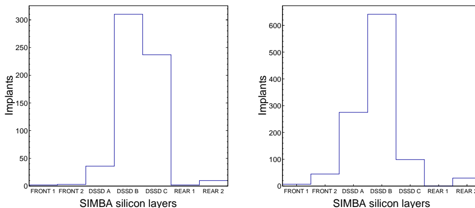
Figure 3.10: SIMBA implantation depth for ^{209}\text{Hg} (left) and ^{213}\text{Tl} (right). Silicon layers are detailed on X axis and the histogram bars present the number of implants on each one.
