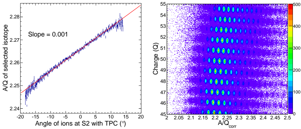
Figure 2.9: Left: Profile of A/Q along the angle measured with the TPC for the selected isotope. The red straight line corresponds to a linear fit. Right: PID after the angle correction.
