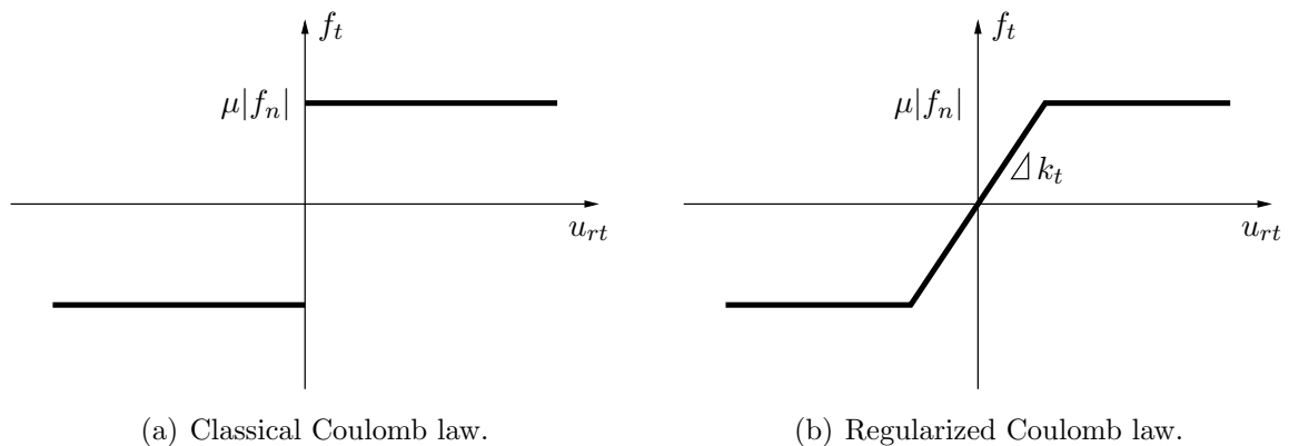
Figure 2.3. Friction force vs. relative tangential displacement.
