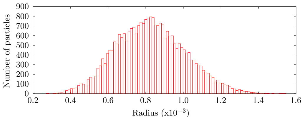
Figure 3.16. Radius distribution in 3D sample with 27.500 spheres.
