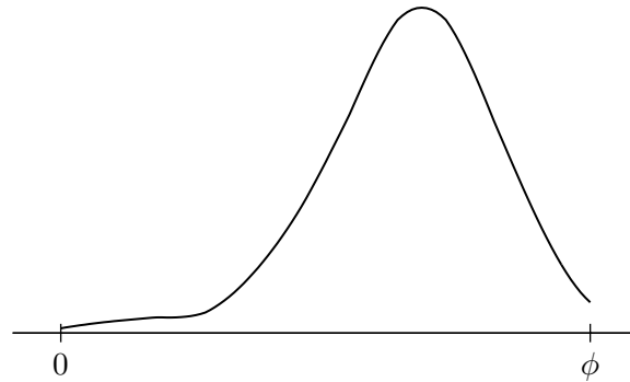
Figure 6.22. Estimated force distribution over disc cutter.
