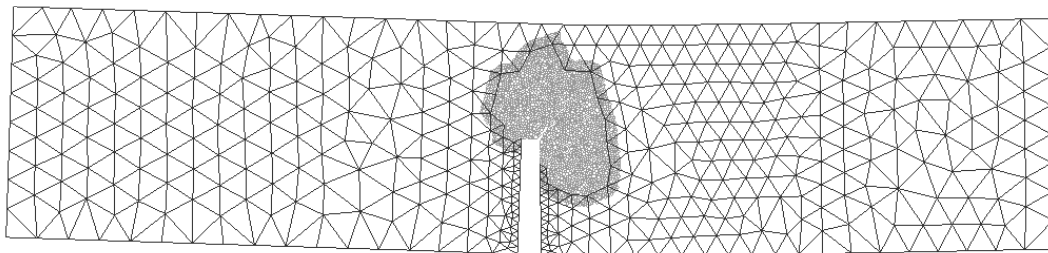
(b) \text{CMOD}=0.0546 \text{ mm}
