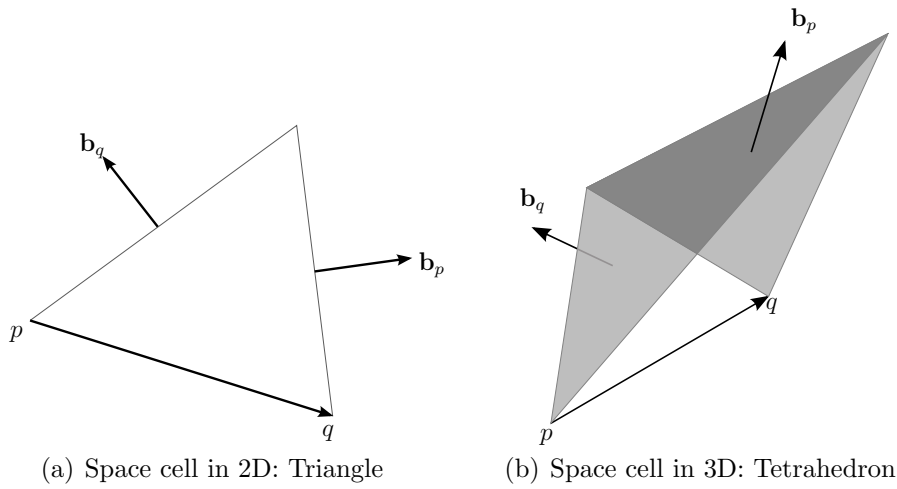
Figure B.2. Sketch of the quantities related with the space cell containing the edge \overline{pq} , with the area vectors \mathbf{b}_q and \mathbf{b}_p .
