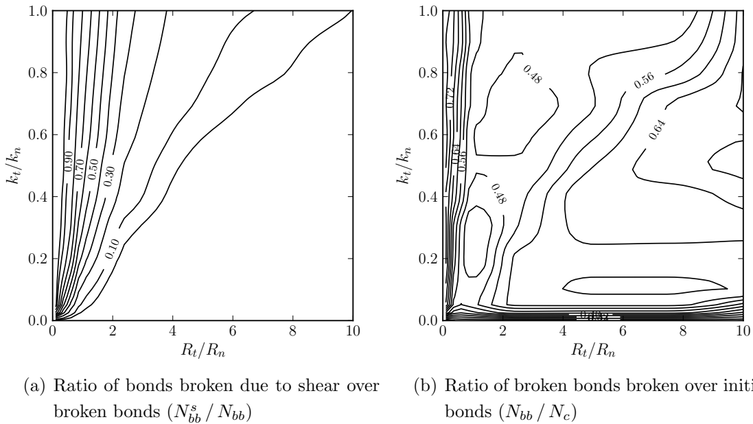
Figure 4.35. Broken bonds for different values of k_t/k_n and R_t/R_n in 3D UCS test.
