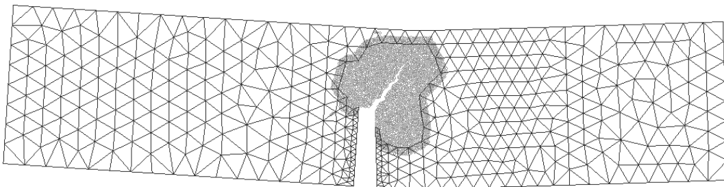
(c) \text{CMOD}=0.1245 \text{ mm}
