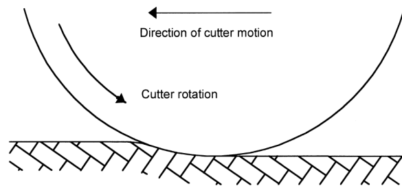
Figure 6.2. A rolling cutter machining a rock surface.
