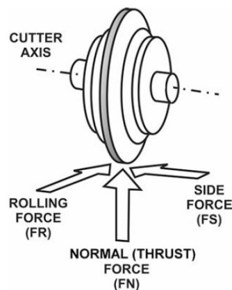
Figure 6.3. Individual force acting on a disc cutter.
