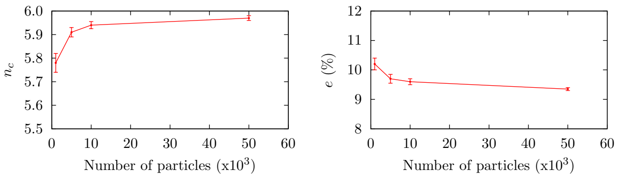
Figure 3.12. Coordination number and porosity for different number of cylindrical particles.
