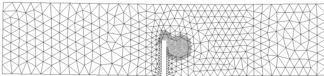
(a) \text{CMOD}=0.0140 \text{ mm}
