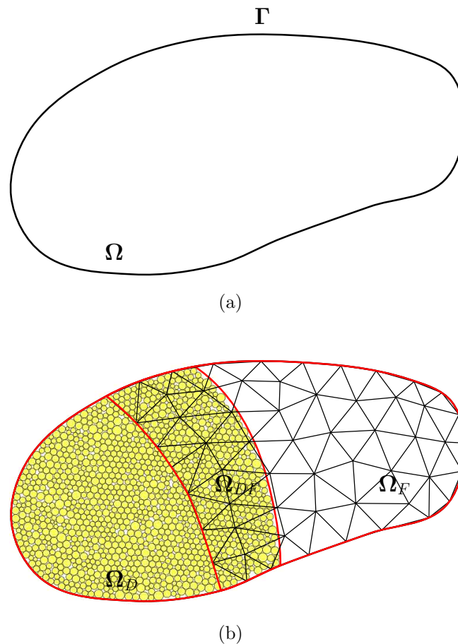
Figure 5.1. Overlap region between DEM and FEM subdomains.
