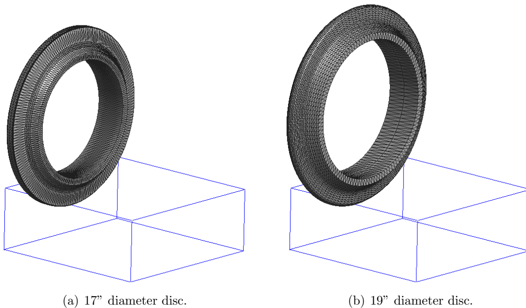
Figure 6.7. Discretization of disc cutters.
