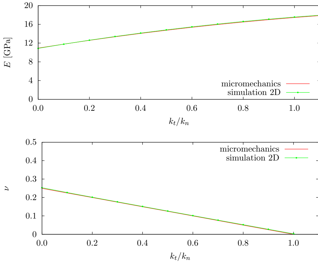
Figure 4.6. Comparison of Young modulus and Poisson's ratio estimated with micromechanics and simulations in specimen 2D.
