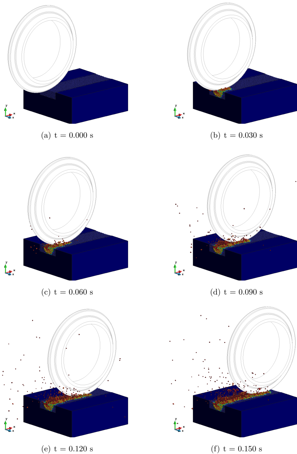
Figure 6.12. Evolution of damage in the LCM test with unrelieved material 1 and ring of 19".
