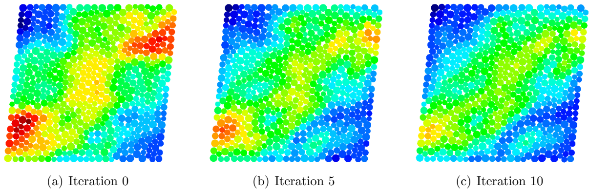
Figure 5.22. Maximum principal stress after different numbers of iterations over the contact forces.
