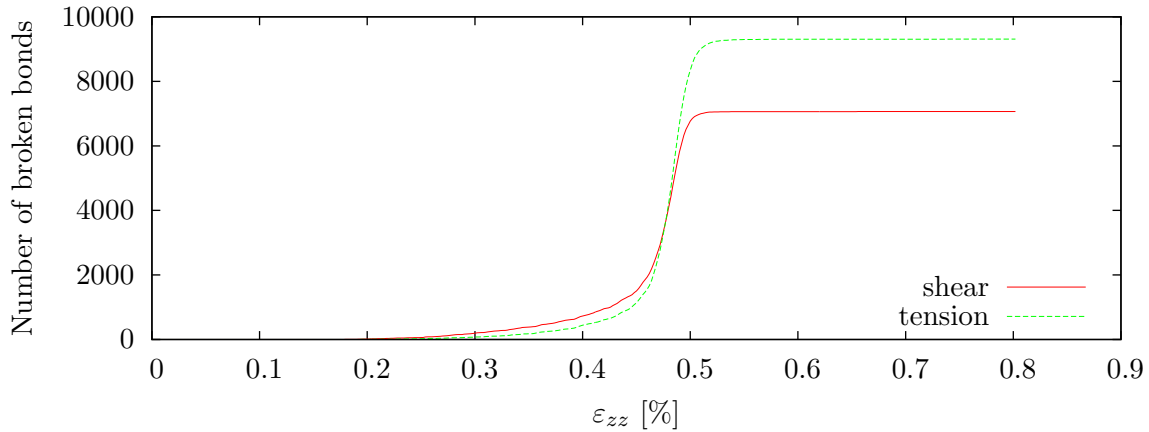
Figure 4.15. Evolution of the broken bonds during the 3D UCS test of specimen 1, with k_t/k_n = 0.30 and R_t/R_n=1 .
