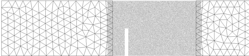
Figure 5.10. Mixed-mode bending beam with a notch. DEM/FEM coupled mesh.
