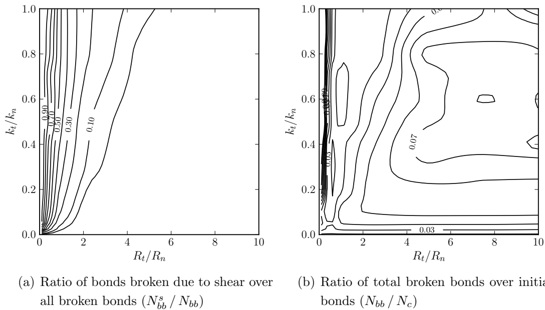
Figure 4.29. Bonds broken for different values of k_t/k_n and R_t/R_n in 2D BTS test.
