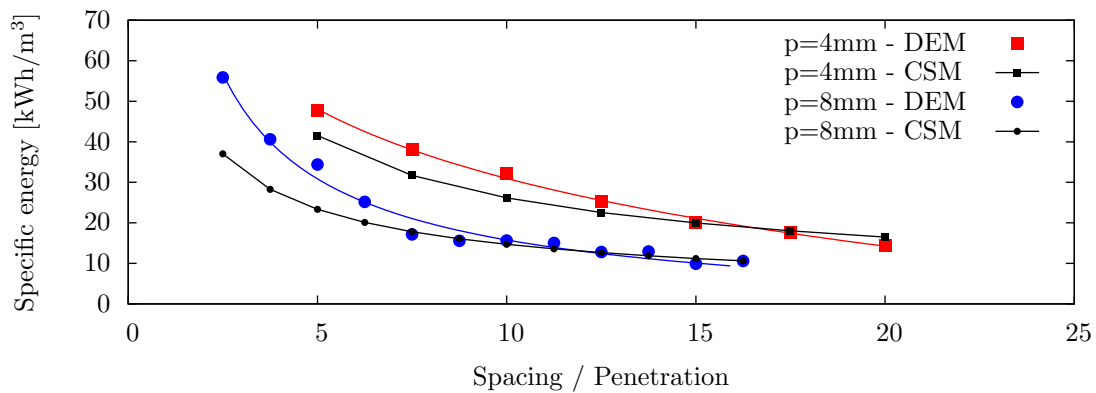
Figure 6.37. Specific energy for different spacing and penetration depths in LCM test with material 1 and ring of 19”.
