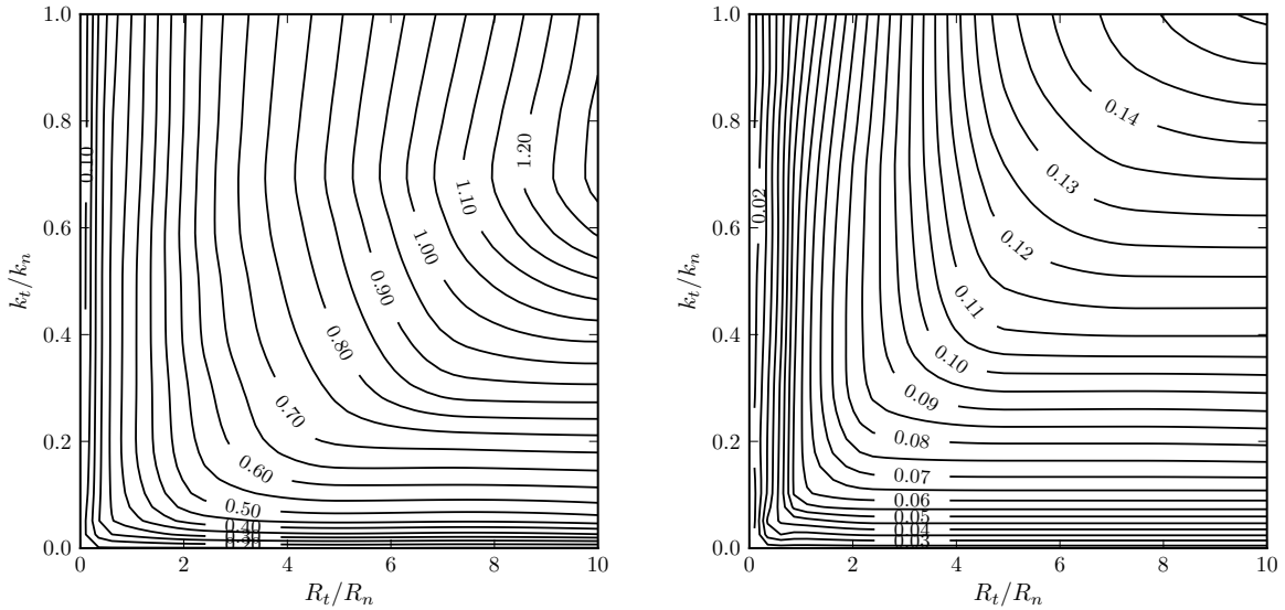
(a) Dimensionless scale function of compressive strength ( \hat{\Psi}_c^{2D} ) (b) Dimensionless scale function of tensile strength ( \hat{\Psi}_t^{2D} )
