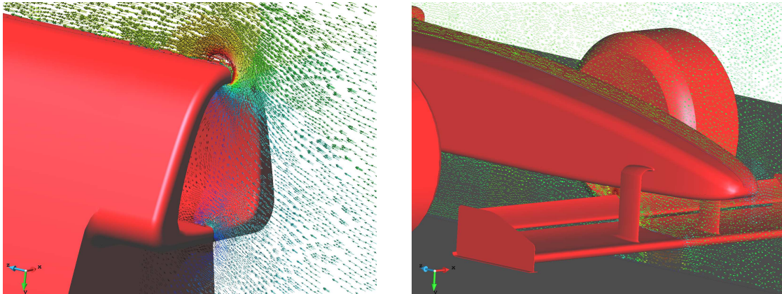
Figure 4.11: Race car test – details of the velocity solution on the finer mesh.
