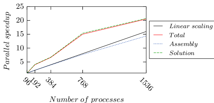
Figure 4.7: Inflatable structure test – parallel speedup for the 35 million elements.
