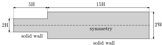
Figure 5.25: Sudden expansion – geometry.
