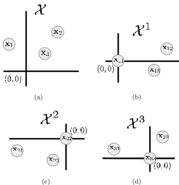
Figure 8.4: The entire point-set \mathcal{X} (a) and, the descriptors \mathcal{X}^1 (b), \mathcal{X}^2 (c) and \mathcal{X}^3 (d), that represent the spatial distribution of the point-sets around their new origins \mathbf{x}_1 , \mathbf{x}_2 and \mathbf{x}_3 , respectively.
