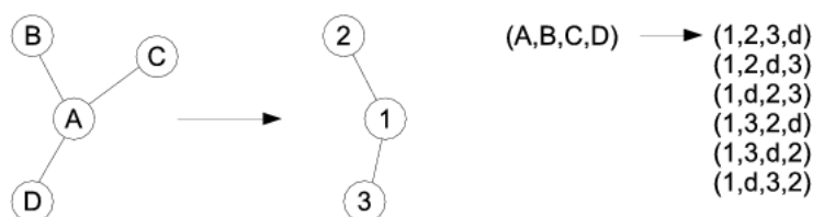
Figure 4.2: Shown in the left-hand side, there are the representations of a clique in the data-graph and a clique in the model-graph. Shown in the right-hand side, there are the string corresponding to the data-graph clique (starting with the symbol of the central node), and the bunch of SPM generated from the model-graph clique by circularly shifting and padding with dummy nodes so as to match the length of the string of the data-clique. Notice that the relative orientations of the adjacent nodes are preserved in the strings.
