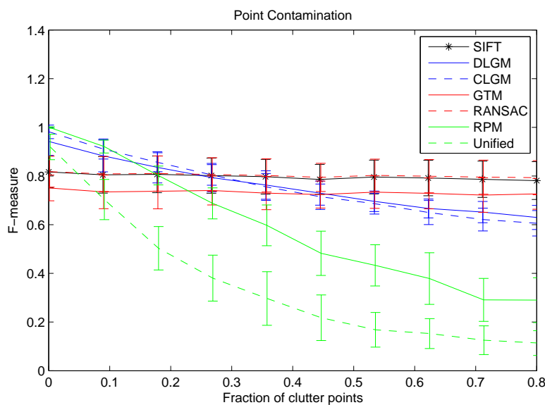
Figure 6.2: Point contamination.
