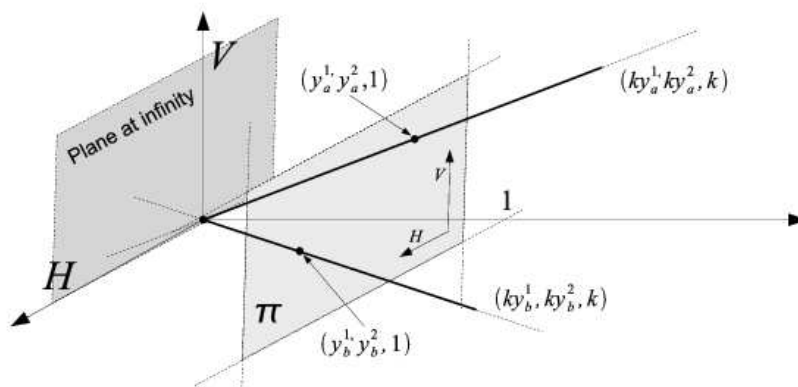
Figure 2.2: Each point in the projective space corresponds to a ray through the origin in \mathbb{R}^3 . The representative of a ray in homogeneous coordinates is taken as the point of intersection of the ray with plane \pi . A ray lying in the plane at infinity does not intersect with plane \pi and hence has no homogeneous representation (it involves a division by zero).
