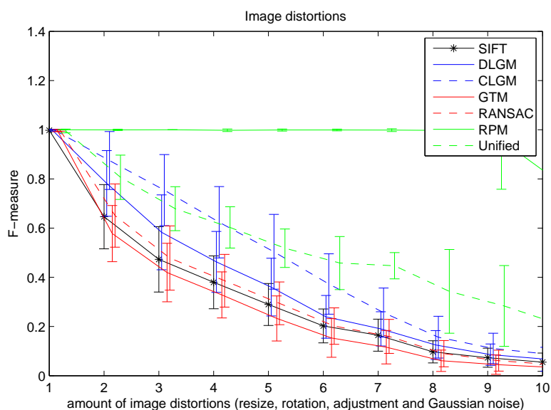
Figure 6.1: Photometric distortions.
