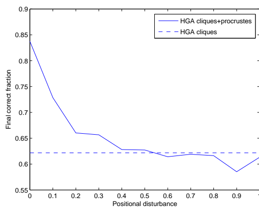
Figure 7.7: Correct assignments fraction with respect to the positional noise.
