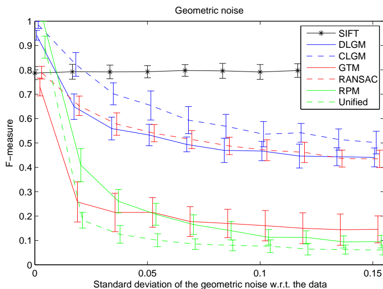
Figure 6.3: Geometric noise.
