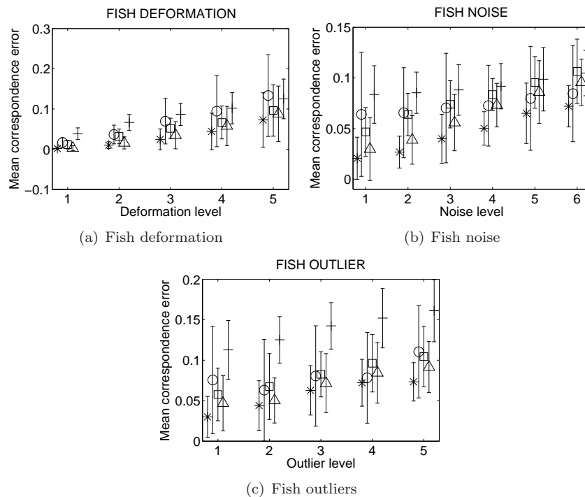
Figure 9.2: Results for the fish (a) deformation, (b) noise, and (c) outlier experiments of (*) our method, (O) our method with P_e = 0.5 (i.e., Softassign Procrustes), (square) Unified approach by Luo & Hancock (2003), (triangle) Graduated Assignment and (-) ICP.
