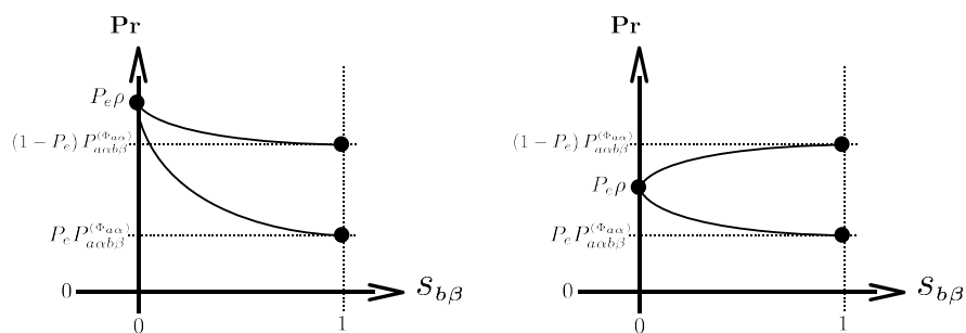
(a) The likelihood value P_{\alpha\alpha b\beta}^{(\Phi_{a\alpha})} is lower than \rho . The density function of equation (8.11) decreases below the outlying threshold ( P_e \rho ) as the correspondence between nodes b and \beta increases. This means that (a, b) is not a plausible relation under the assumption that node a corresponds to \alpha and b to \beta . (b) The density function of equation (8.11) only increases as the correspondence indicator increases in the case of structural consistency (i.e., D_{ab} = 1 \wedge M_{\alpha\beta} = 1 ). In this case, structural consistency makes the difference between considering (a, b) \rightarrow (\alpha, \beta) a plausible mapping or not.
