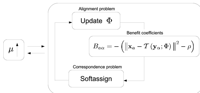
Figure 3.3: Overview of the Robust Point Matching algorithm. The procedure iterates until convergence or until \mu reaches a predefined threshold.
