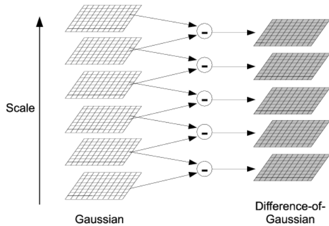
Figure 1.5: The initial image is successively convolved with Gaussians (i.e. blurred) to produce the set of scale space images shown on the left. Adjacent images are subtracted to produce the Difference-of-Gaussian images on the right.
