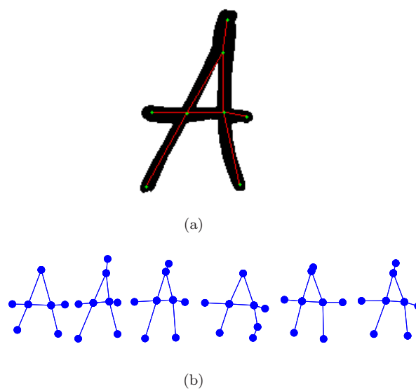
Figure 7.1: (a) example of a graph extraction from a handwritten character and, (b) several graphs from the same class.
