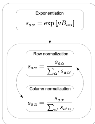
Figure 3.2: Overview of the Softassign procedure.
