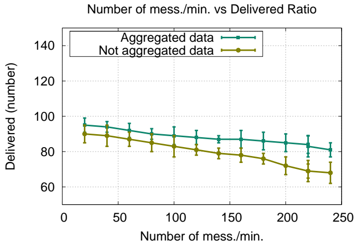
Figure 7.6: Delivery ratio studied as a function of the number of messages in a scenario that uses the custodian block code extension to deploy aggregation code versus another scenario which does not.
