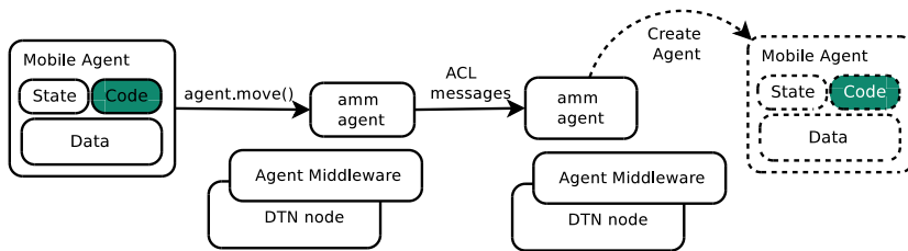
Figure 4.1: Mobile agent migration. A mobile agent migrates from one mobile agent middleware with its state, code and data, to another mobile agent middleware. FIPA-ACL messages are designed to contain all data necessary for agent communication.
