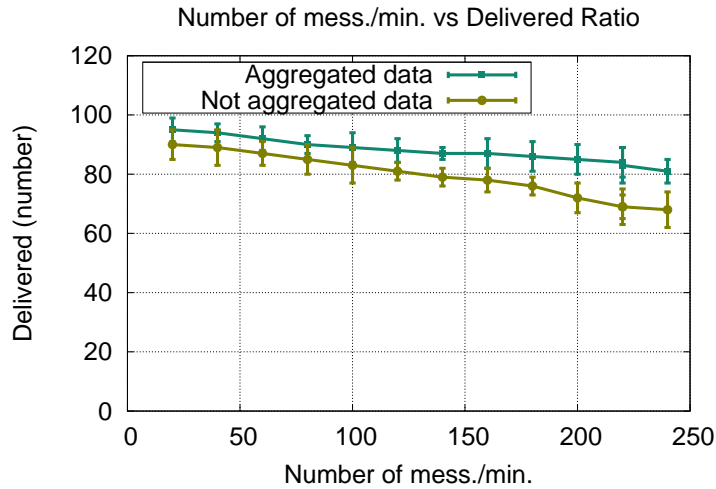
Figure 5.11: Delivery ratio as a function of the number of messages. Aggregated data improves significantly the delivery ratio.
