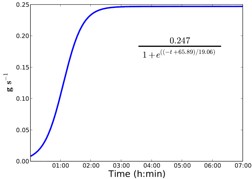
Fig. 2.6. Logistic function for the condensation curve.
