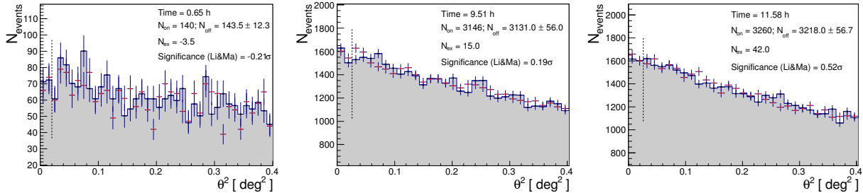
Figure 10.1: Distribution of the squared distance between the nominal and reconstructed source position (red points) and the background estimation (shaded region) in the MAGIC observations of the three objects: YY Her (left panel, E \gtrsim 70 GeV), ASASSN-13ax (middle panel, E \gtrsim 110 GeV) and V339 Del (right panel, E \gtrsim 80 GeV).
