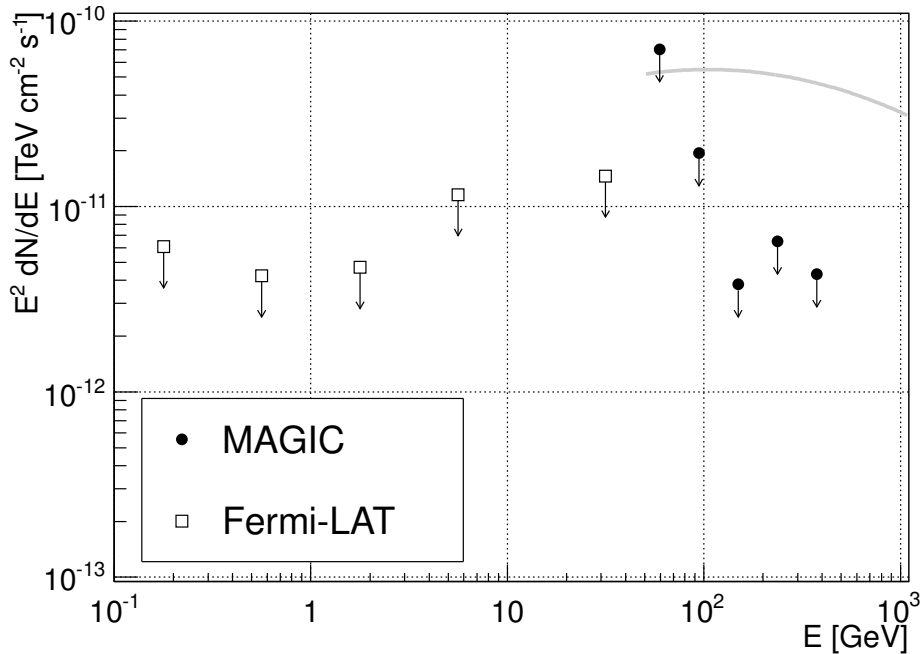
Figure 10.3: Differential ULs on the flux from YY Her measured by MAGIC (filled circles) and Fermi -LAT (empty squares). For comparison, a spectrum of Crab Nebula is shown with a grey curve.
