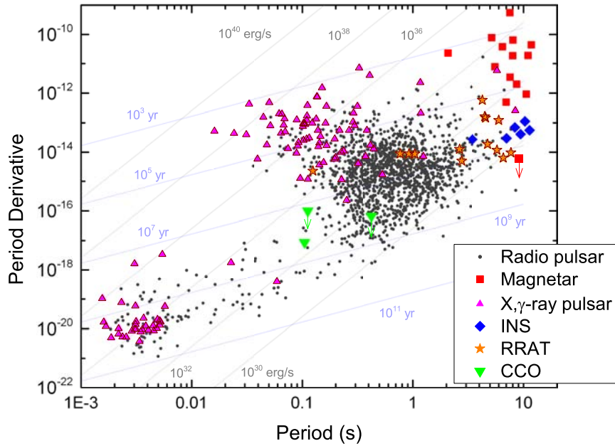
Figure 5.5: Plot of P vs. \dot{P} for the currently known rotation-powered pulsars, INS, CCO, Rotating Radio Transients (RRATs) and magnetars. Lines of constant characteristic age, P / 2\dot{P} , and dipole spin-down luminosity, \dot{E}_{\text{sd}} , are also drawn. Plot from (Harding 2013).
