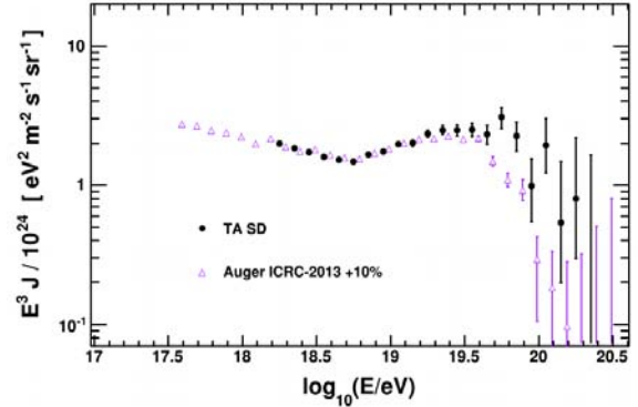
Figure 1.2: Auger and Telescope Array results for the CR flux at the highest energies measured. From Matthews, J. (2014).
