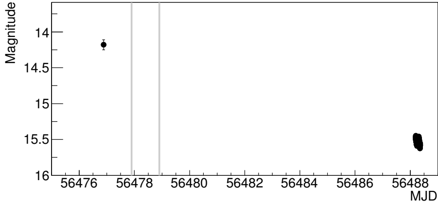
Figure 10.4: Optical observations in V band of ASASSN-13ax during the outburst in July 2013. The data points are obtained from AAVSO-LCG service. The grey vertical line shows the two observation nights with MAGIC .
