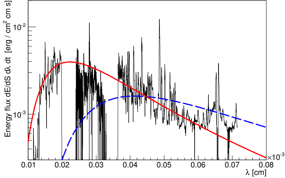
Figure 10.7: Thin black lines: optical spectrum of V339 obtained by NOT on MJD 56532 (above 3500 Å) and scaled UV spectrum of OS And nova in SWP and LWP ranges (points obtained from Shore, S. N. 2015, in preparation). Thick lines: the spectra are overlaid with simple black-body photosphere modelings of Metzger et al. (2015) (blue dashed line) and one taking into account also SWP and LWP ranges (red solid line). The assumed distance of V339 Del is 4.5 kpc.
