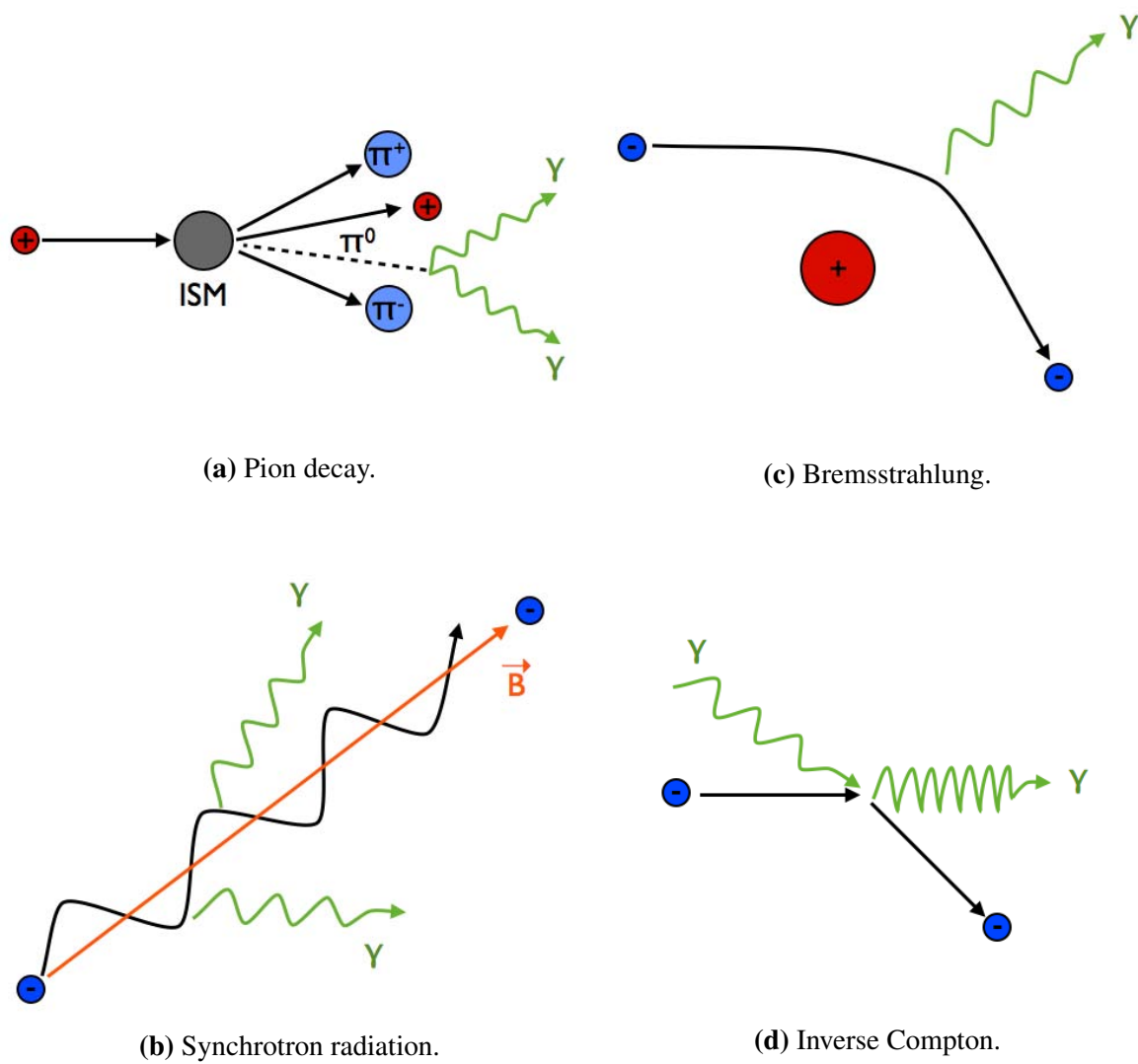
Figure 1.4: VHE \gamma -ray production mechanisms.
