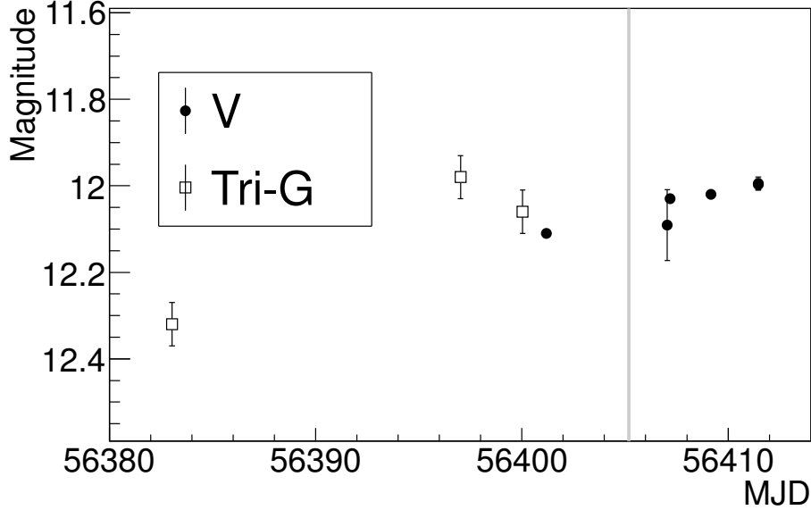
Figure 10.2: Optical observations of YY Her during the outburst in April 2013. The data points in V (filled circles) and Tri-G (empty squares) range are obtained from AAVSO-LCG service. The grey vertical line shows the observation night with MAGIC .
