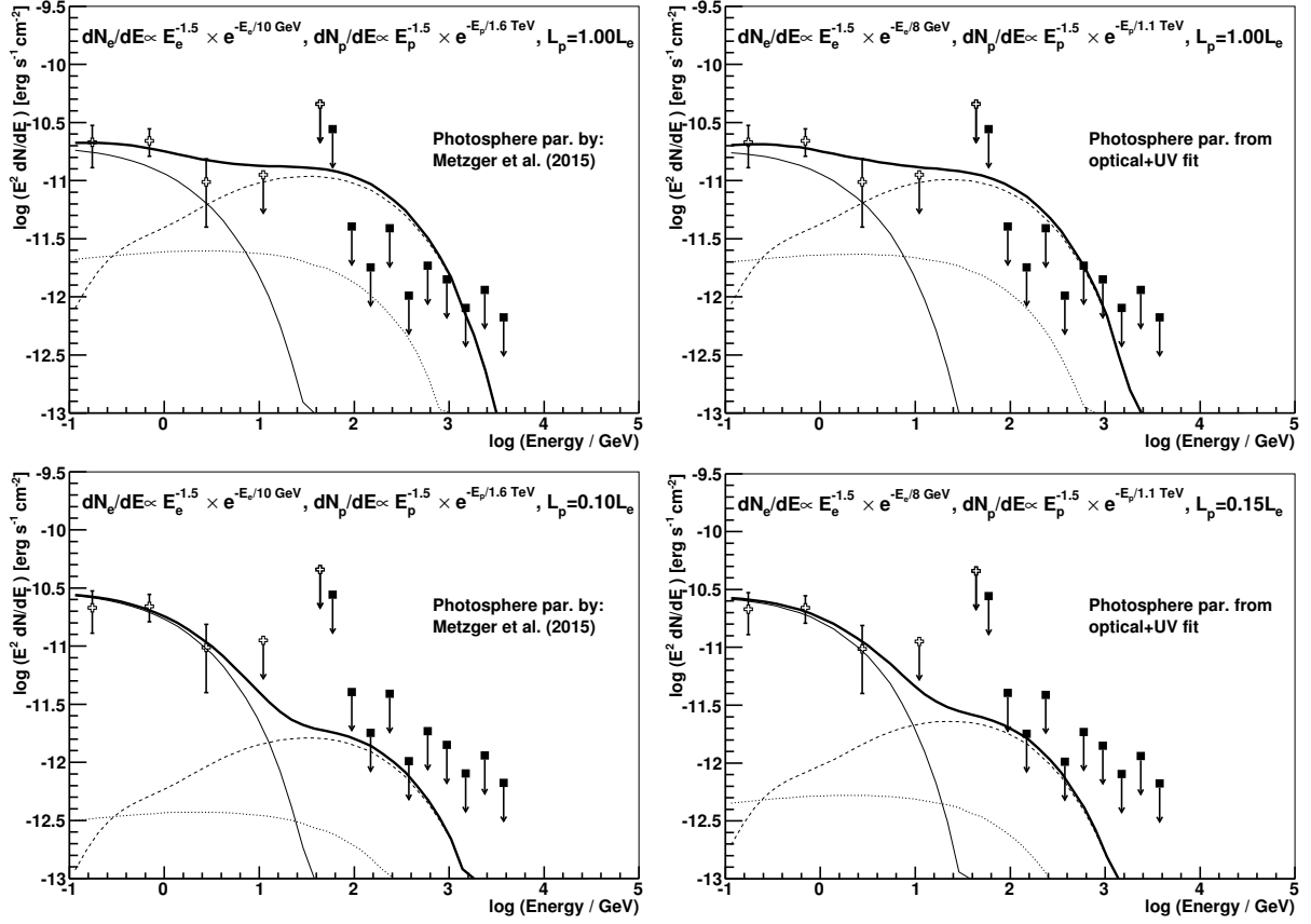
Figure 10.8: Differential ULs on the flux from V339 Del measured by MAGIC (filled squares) and the flux measured by Fermi -LAT (empty crosses) in the period between MJD 56529 and 56539. The thin solid line shows the IC scattering of thermal photons of the nova’s photosphere. The dashed line shows the gamma rays coming from the decay of \pi^0 from hadronic interactions of the relativistic protons with the nova ejecta. The dotted line shows the contribution of gamma rays coming from IC of e^+e^- originating from \pi^+\pi^- decays. Thick solid lines show the total predicted spectrum. Electrons and protons are injected with a power-law with a spectral index of 1.5 and the cut-offs reported in the figures. Photosphere parameters (see Table 10.3) by Metzger et al. (2015) (left panels) or from optical+UV fit (right panels). Top panels: L_p = L_e , bottom panels for obtained L_p/L_e limits, i.e. L_p = 0.1L_e or L_p = 0.15L_e (see top right corner of panels).
