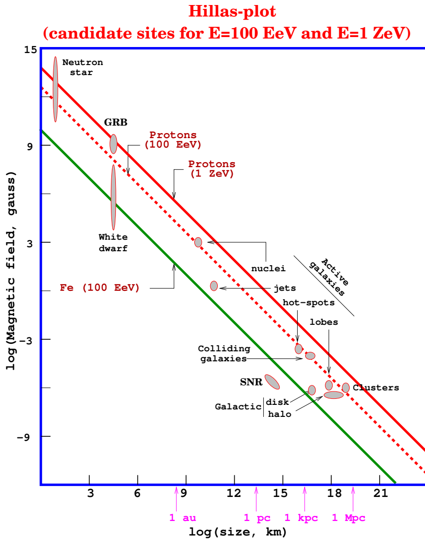
Figure 1.3: Magnetic field and typical size of several potential sources of UHECRs. The lines indicate that the confinement radius requirement for a particular particle with the indicated energy does not exceed the source size. Sources below each line cannot produce CRs with an energy larger than the indicated value. From Hillas (1984).
