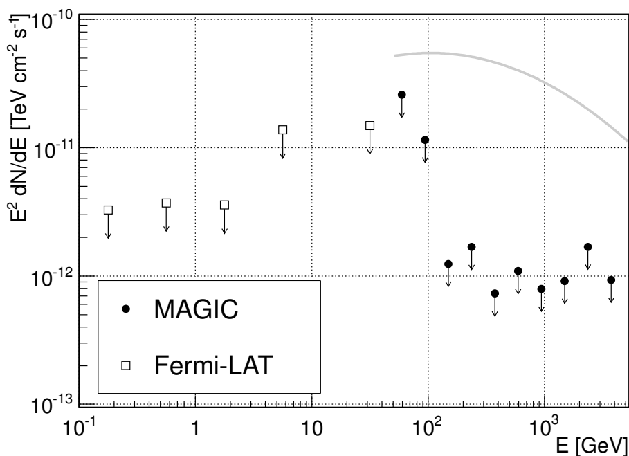
Figure 10.5: Differential ULs on the flux from ASASSN-13ax measured by MAGIC (filled circles) and Fermi -LAT (empty squares). For comparison a spectrum of Crab Nebula is shown with a grey curve.
