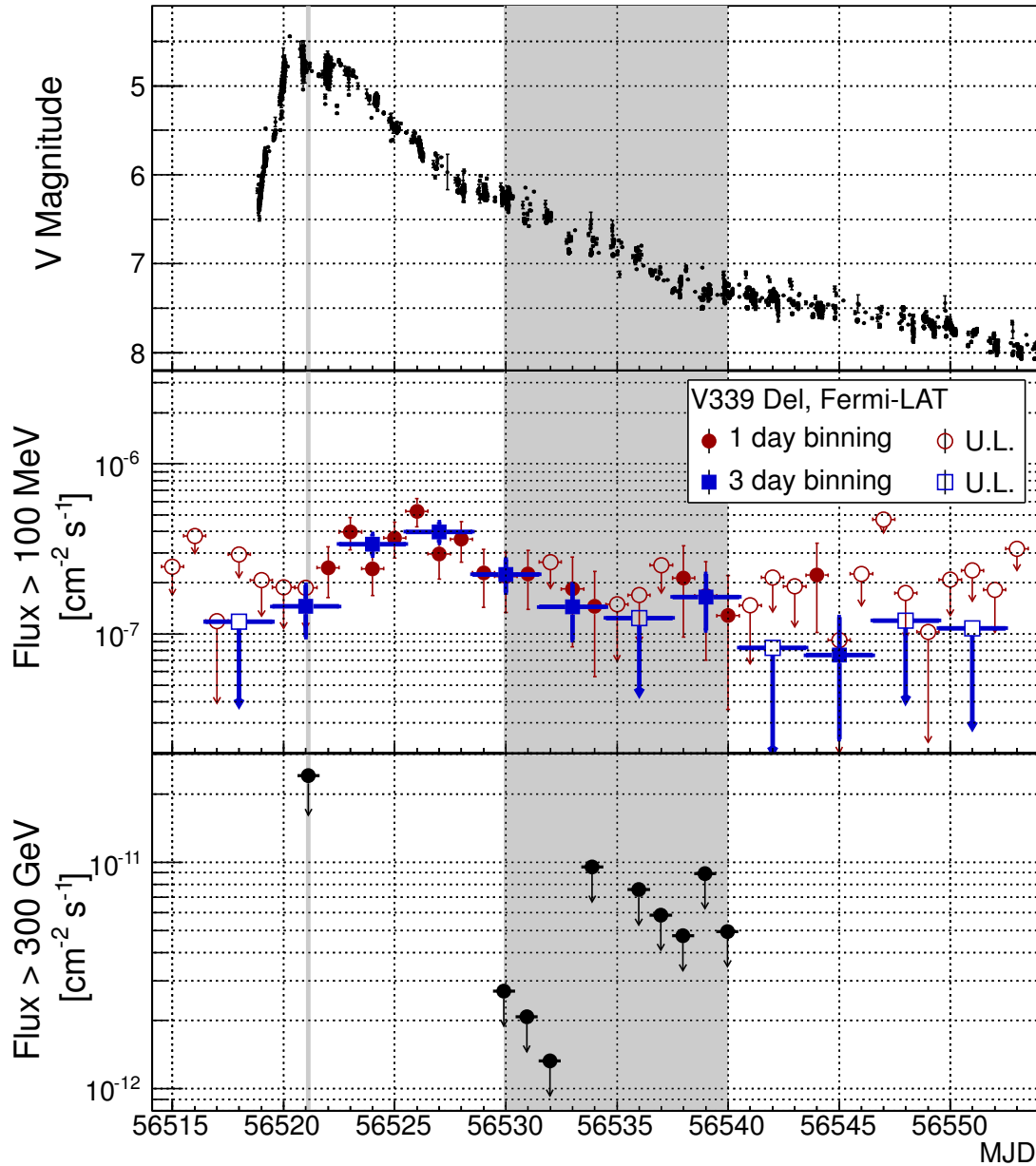
Figure 10.6: Multiwavelength light curve of V339 Del during the outburst in August 2013. Top panel: optical observations in the V band obtained from AAVSO-LCG 1 service. Middle panel: Fermi -LAT flux (filled symbols) and ULs (empty symbols) above 100 MeV in 1-day (circles, thin red lines) or 3-day (squares, thick blue lines). A 95% C.L. flux UL is shown for time bins with TS < 4 . Bottom panel: UL on the flux above 300 GeV observed with MAGIC telescopes. The grey bands show the observation nights with MAGIC .
