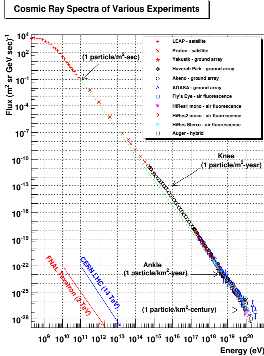
Figure 1.1: Cosmic-ray spectrum observed from the Earth. From Hanlon (2010).
