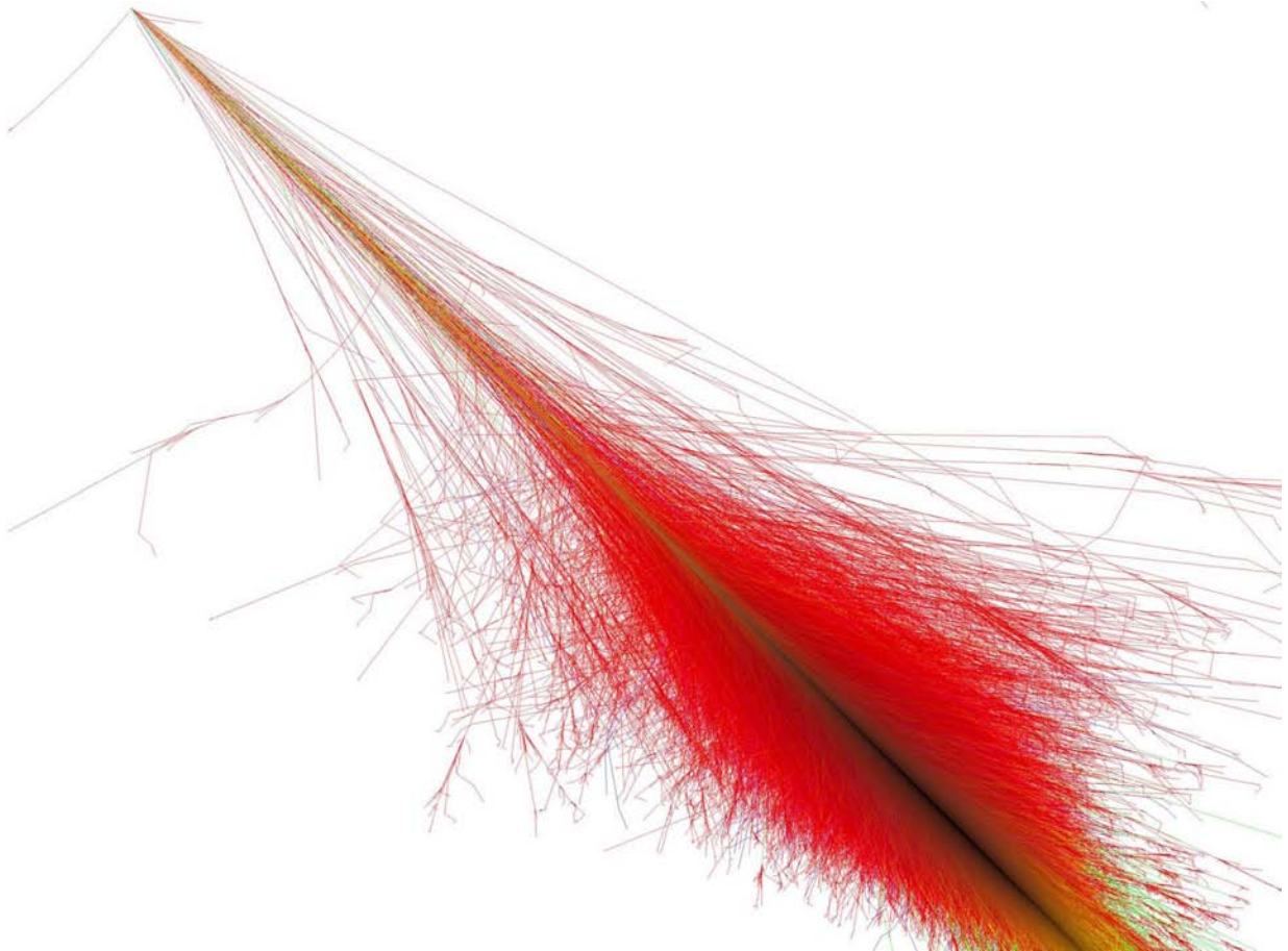
Figure I: Air shower. Credit: Fabian Schmidt.
