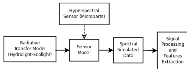
Figure 1: Proposed methodology to analyse hyperspectral data.
