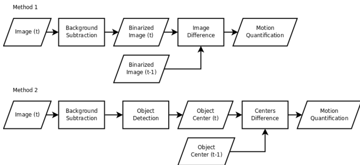
Fig. 1: Work flow of the two methods.
