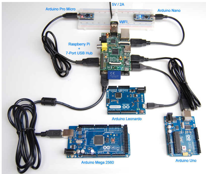
Figure 6.5: Raspberry Pi connected to five different Arduino boards with the help of a USB hub. With permission from UUGear.com ©2015 (UUGear, 2015).
