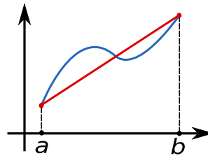
Figure 5.1: Example of application of the trapezoidal rule. The function f(x) (in blue) is approximated by a linear function (in red) between the points a , b .
