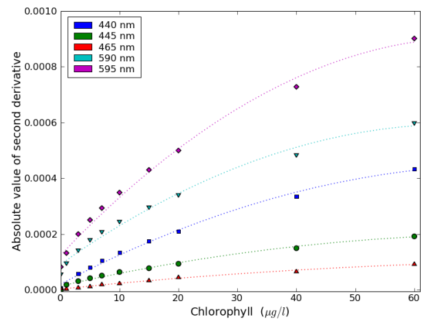
Figure 2: Relationship between chlorophyll a concentration and height of the second derivative at several wavelengths of attenuation factor ( K d ) at 4 m depth.
