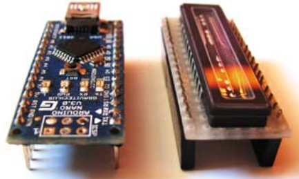
(b) Arduino Nano with Spectruino shield. With permission from Andrej Mosat ©2012 (mySpectral, 2015).
