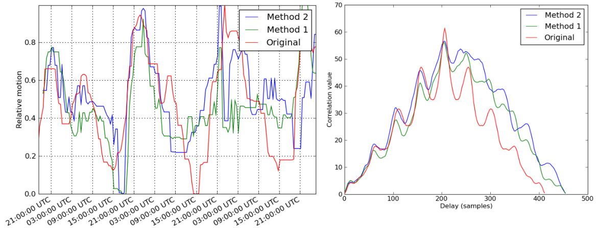
Fig. 2: (left) Monitored activity for a single specimen, with the manual sampling and the automated methods. (right) Cross-correlation of the manual (original) method with itself, and the manual method versus the automated methods.
