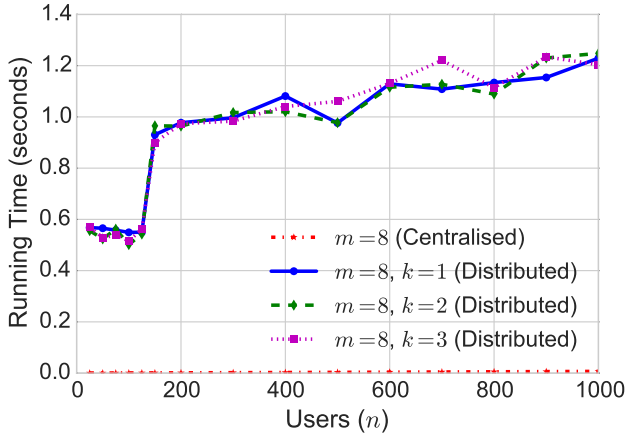
Figure 5.11: Running time for double auction
