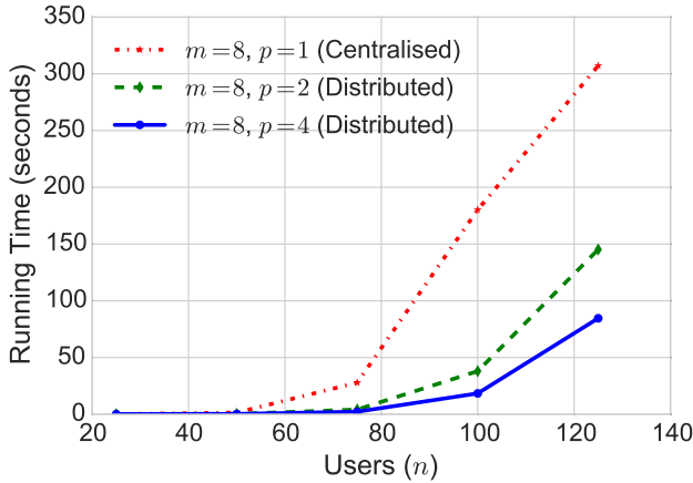
Figure 5.12: Running time for standard auction
