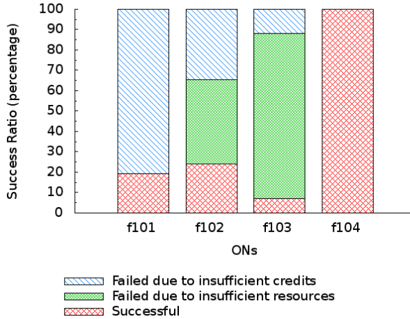
Figure 4.8: Ratio of fulfilled and rejected requests
