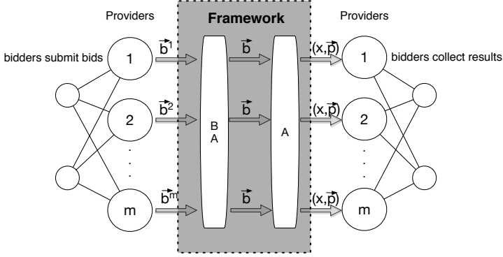
Figure 5.8: Framework: Bid Agreement (BA) and Allocator (A)
