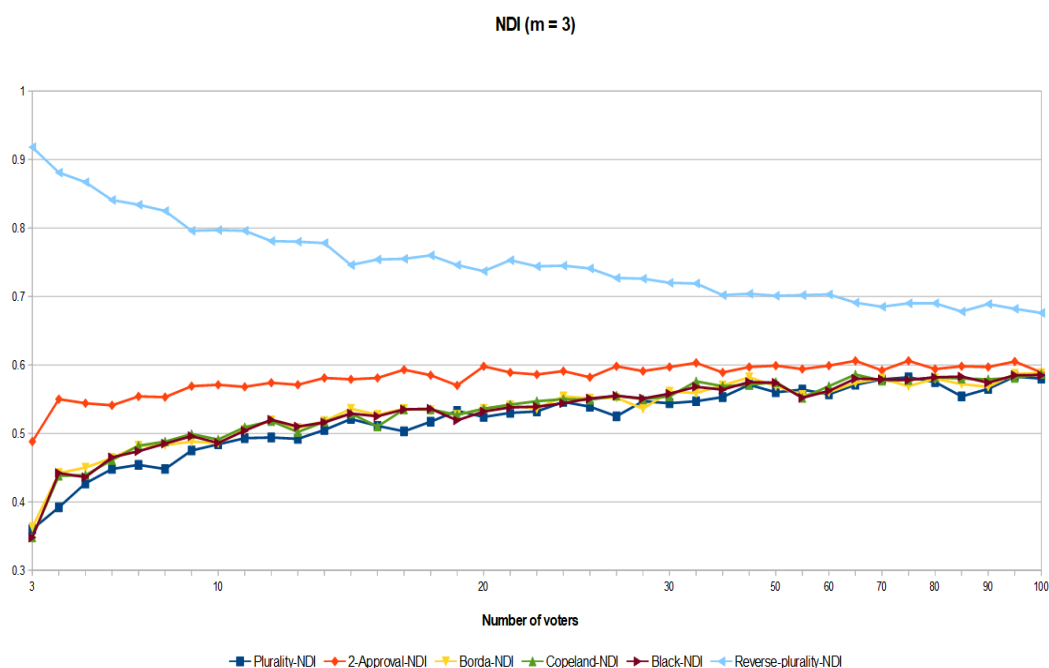
Figure 5.1: Non-dictatorship indices in case of three alternatives
