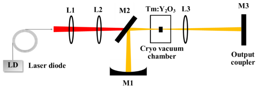
Figure 4-1 Sketch of the CW laser setup. LD – pump laser diode; L1 & L2 - achromatic lenses; M1 – plano-concave cavity mirror; M2 - dichroic mirror; L3 – plano-convex thin lens; M3 – output coupler.
