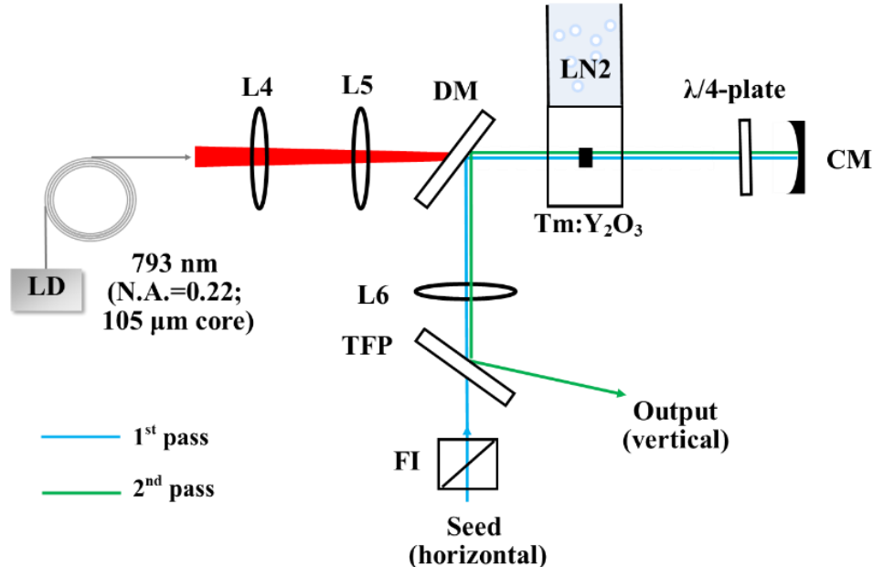
Figure 6-1 Sketch of the double-pass amplifier setup. Red line: pump radiation, blue line: the 1 st laser pass, green line: the 2 nd laser pass. L4 & L5: AR coated achromatic lenses; FI: Faraday isolator; TFP: thin film polarizer; L6: AR coated thin lens; DM: dichroic mirror; CM: curved mirror.
