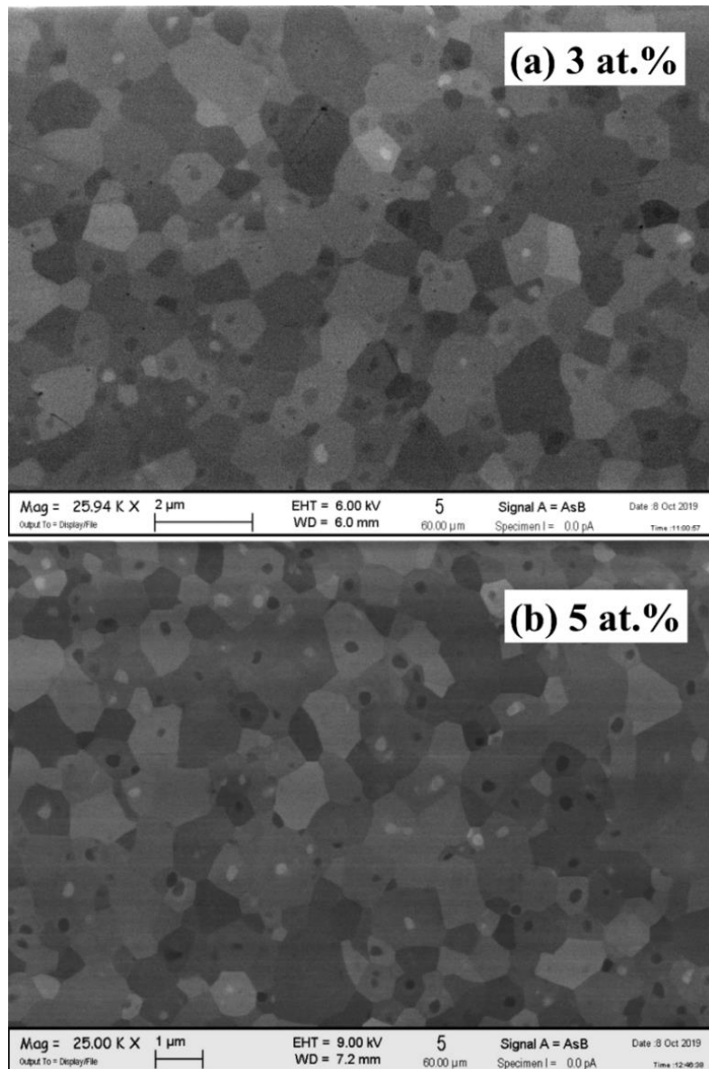
Figure 2-4 The SEM microstructure of (a) 3 and (b) 5 at.% \text{Tm}:\text{Y}_2\text{O}_3 transparent ceramic samples, measured from the polished surface.
