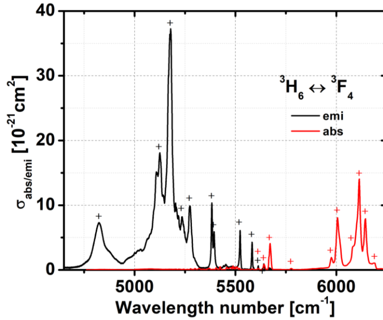
Figure 3-12 Low temperature (6 K) optical absorption and emission between energy levels 3 H 6 and 3 F 4 .
