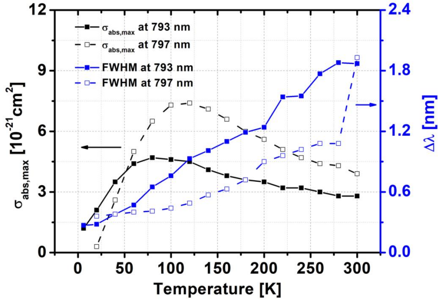
Figure 3-10 Peak values (black) and FWHM (blue) of the absorption cross-section peaks around 793 and 797 nm, plotted as a function of temperature.
