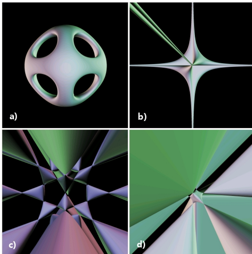
Figure 7.5: Tested surfaces: a) orthochirle, b) steiner, c) bath, d) weird.
