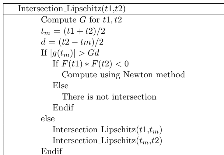
Figure 4.12: Intersection test using Lipschitz constants.
