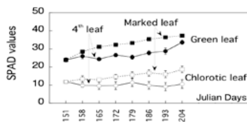
Fig. 4. Changes in leaf SPAD values in Fe-sufficient leaves (green; black symbols) and Fe-deficient leaves (chlorotic; white symbols) using two different leaf samples. Developed leaves in the distal branch tip were marked at the beginning of the experiment with colour tape and SPAD was measured in the same leaves throughout the experiment (marked leaves; squares) or in leaves at the 4th position in the branch (circles) (in all cases n = 6 trees).
