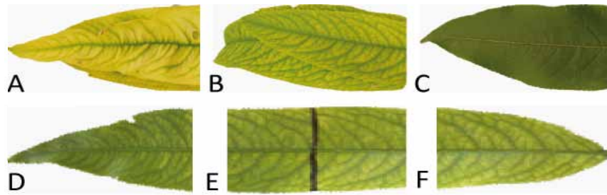
Figure 3.7. Peach tree leaves used for the Chl fluorescence measurements. (A) Severely chlorotic leaf, with a very advanced chlorosis status, taken from the distal part of the shoot; (B) Fe-deficient leaf taken at the 4-5 th position in the shoot, one week after treatment by dipping the upper half of the leaf in a solution containing 2 mM FeSO 4 and 0.1% surfactant; (C) Positive control: Fe-sufficient leaves taken in the same position in the shoot but from a Fe-sufficient tree; (D) distal part of an Fe-treated leaf; (E) middle part of an Fe-treated leaf, showing the black line delimiting the treatment area; and (F) basal part of an Fe-treated leaf.
