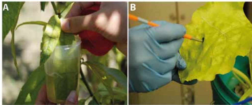
Figure 3.2. Treatment of the distal half part of (A) peach leaves by dipping and (B) sugar beet leaves using a paint brush with a solution containing 2 mM \text{FeSO}_4 and 0.1% surfactant.
