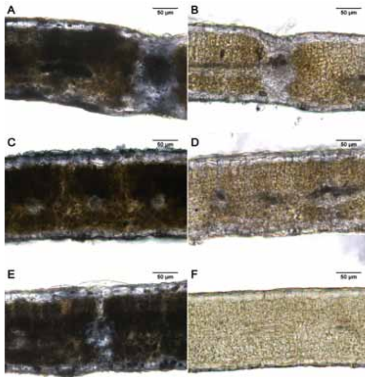
Figure 3.5. Iron staining (Perls-DAB) in leaf peach tree transversal sections: (A) Fe-sufficient control; (B) Fe-deficient chlorotic; (C) distal treated leaf part (2 mM \text{FeSO}_4 with 0.1% surfactant); (D) basal untreated leaf part in the same leaves used for C; (E) leaves of a soil fertilized tree (Sequestrene, 50 g/tree); and (F) negative control.
