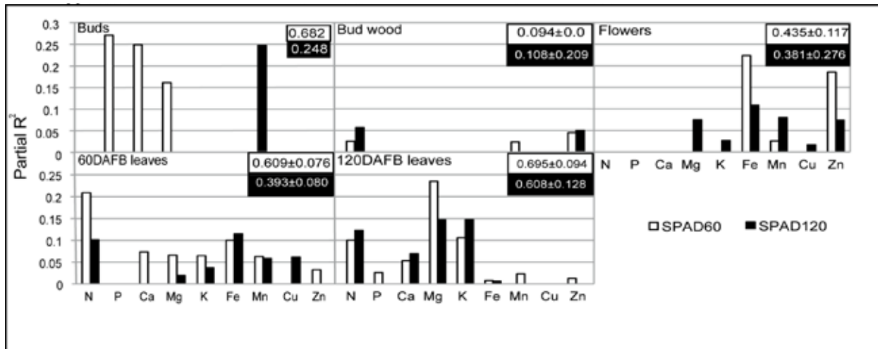
Fig. 6 Determination coefficients (partial R^2 ) between pear tree nutrients in different tissues and SPAD values at 60 and 120 DAFB. Coefficients of determination for the stepwise multiple analyses (global R^2 ) are shown in each graph in insets (white
