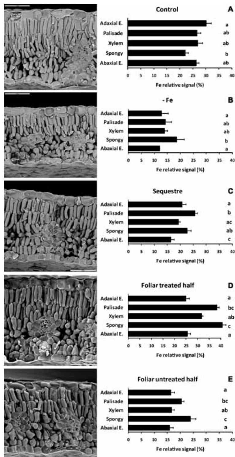
Figure 3.6. LT-SEM micrographs (left panels) and EDX analysis (spot mode, right panels) of transversal sections obtained by cryo-fracture from peach tree leaves: (A) Fe-sufficient control; (B) Fe-deficient chlorotic; (C) soil fertilized (Sequestrene, 50 g per tree); (D) distal Fe-treated leaf part (2 mM FeSO 4 with 0.1% surfactant); and (E) basal untreated leaf part in the same leaves used for D. Relative Fe signals are means ( \pm SE). Significant differences among plant tissues are indicated by different letters ( p \leq 0.05 ; n = 8 ). Bars in the images are 50 \mu m.
