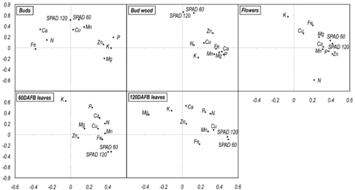
Fig. 4 Principal component analysis of the pear tree nutrient database. Nutrient concentrations measured in different years in bud wood, buds, flowers and leaves at 60 and 120 DAFB leaves, as well as SPAD values at 60 and 120 DAFB were included as variables in the analysis. The first principal component explained 35, 33, 33, 32 and 30% of the total
