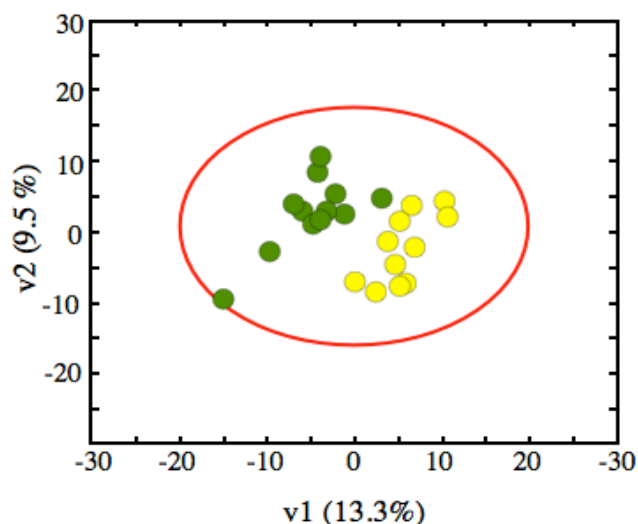
Figure 4.4. Partial least square (PLS) analysis of xylem sap and leaf extract metabolites as affected by Fe deficiency. Score scatter plot of PLS vector1 (v1) vs. PLS vector2 (v2) of all detected metabolites (identified ones plus unknowns) in control (green circles) and Fe-deficient (yellow circles) sample. The percentage of variability explained by each vector is indicated in parenthesis in the corresponding axes.
