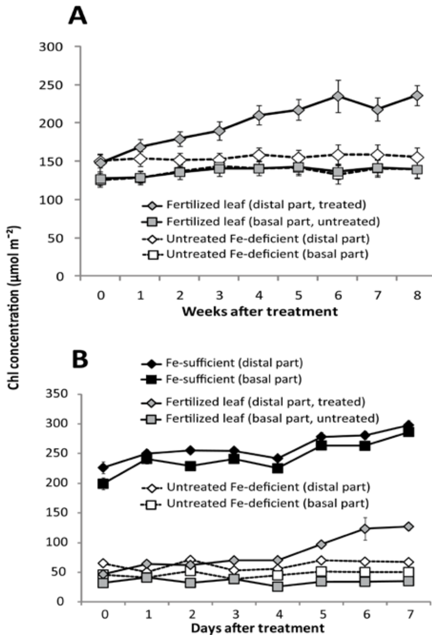
Figure 3.3. Time course of the changes in leaf Chl concentration in peach tree (A) and sugar beet (B). The treatment was carried out with a solution containing 2 mM \text{FeSO}_4 and 0.1% surfactant. In peach leaves, foliar treatment was made at weeks 0 and 4 and SPAD index was measured each week. In sugar beet leaves, treatment was made at days 0 and 2 and SPAD was measured daily. Data are means \pm SE ( n = 12 , 4 plants per bucket).
