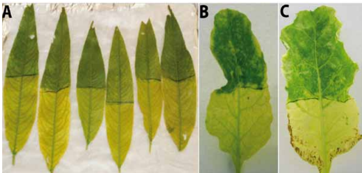
Figure 3.4. Images of peach tree leaves 8 weeks after the first foliar Fe treatment (A) and two different sugar beet leaves 8 days after the first treatment (B and C). The green areas are the result of treatments with a solution containing 2 mM FeSO 4 and 0.1% surfactant.
