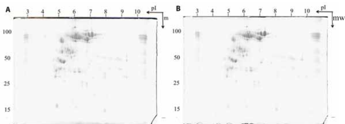
Figure 4.6. 2D electrophoresis gels obtained from Fe-sufficient (A) and Fe-deficient (B) peach xylem sap samples. Xylem sap proteins were precipitated with 10% TCA, and 70 \mu\text{g} of solubilized xylem sap proteins were separated in a first dimension by IEF (3-10 strip) and then in a second dimension by SDS-PAGE (12%) buffer.
