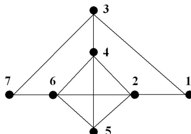
Figure 3.1: \{2, 6\} is a powerful (-2) -alliance and \{2, 3, 4, 6\} is a global powerful (-1) -alliance.
