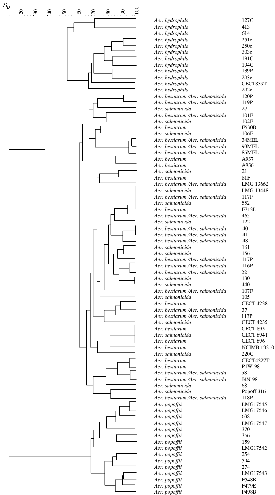
Figure 2. S_D /UPGMA cluster analysis based on the combined Hinf I-CfoI and Hinf I-TaqI restriction patterns of amplified 16S-23S ISR of the 76 of the Aeromonas strains identified by the 16S rDNA RFLP method.
