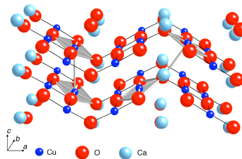
FIG. 1: Crystal structure of \text{CaCu}_2\text{O}_3 . Thick grey lines connect the cluster atoms used to compute the two different interplane interactions. The c , 1 and c , 2 interaction paths are schematically depicted on the left- and right-side, respectively.
